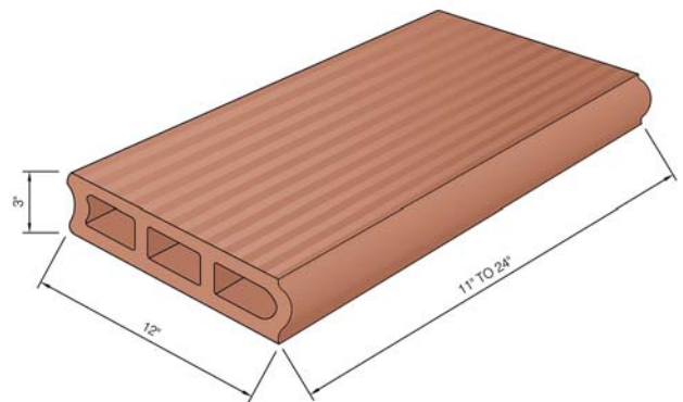
Figure 1 – With the general appearance of a closed book, these units were popular during the late 1800s and early 1900s.
