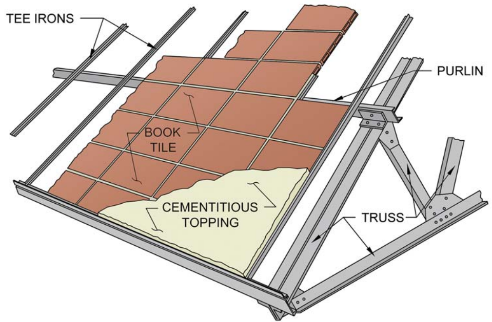
Figure 4 – The common arrangement of tiles nested onto sloped steel framing. Additional mortar would be struck into joints from the roof (top) side.
